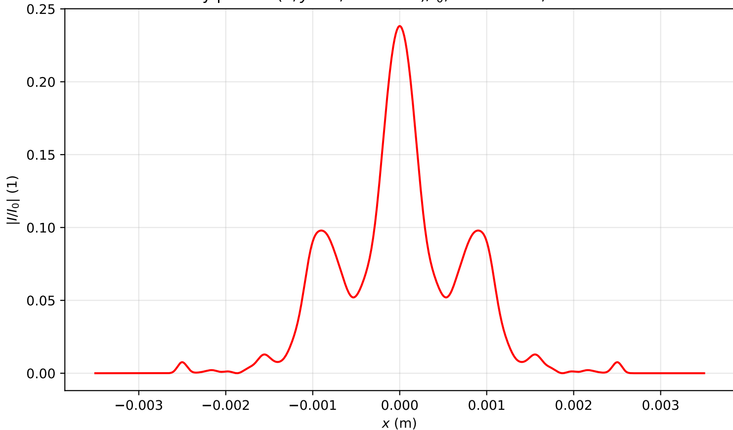
Intensity profile I(x, y = 0, z = 2.388)/I_0 , P_{in}=6.0P_{cr} , artificial time
